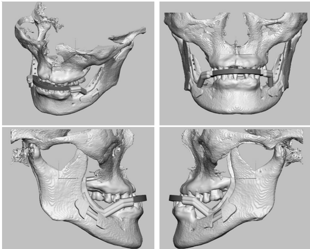
Fig. 3. Design of BSSRO surgical guide. Surgical guide contain information of sawing line and position of inferior alveolar nerve.
