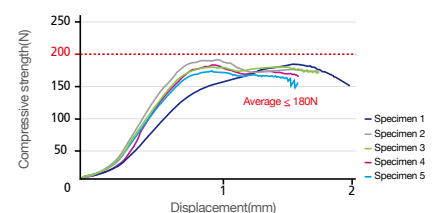
Compressive strength test of Fuse Abutment
